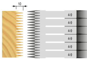
Giunto verticale / Vertical joint / Vertikale Zinkung
